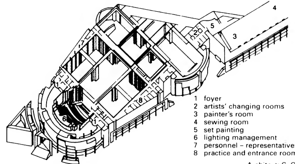
⑦ Opéra Bastille, Paris 1989 Architect: C. Ott
